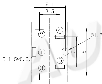
P. C. B LAYOUT
