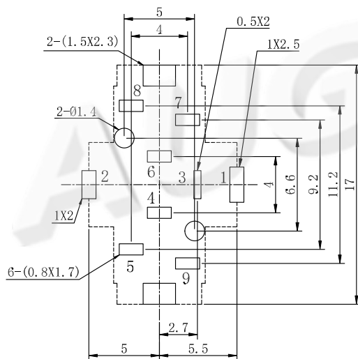
P. C. B LAYOUT
