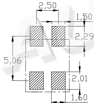
RECOMMENDED PCB LAYOUT TOP VIEW (. XX±0.05)
