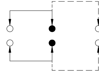
SCHEMATIC (NON-SHORTING)
