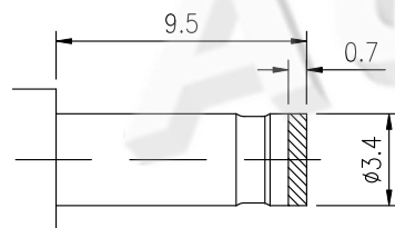
MATE PLUG
