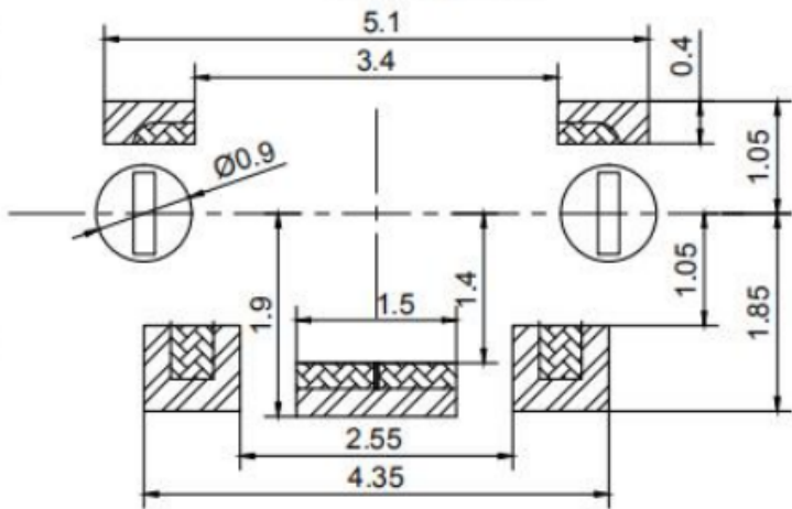
PCB.layout
