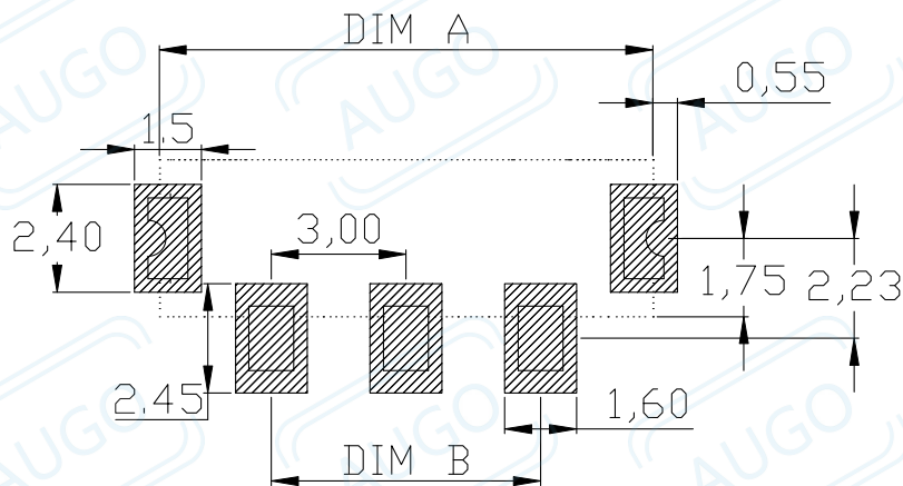
RECOMMENDED PCB LAYOUT TOP VIEW(.XX±0.05)
